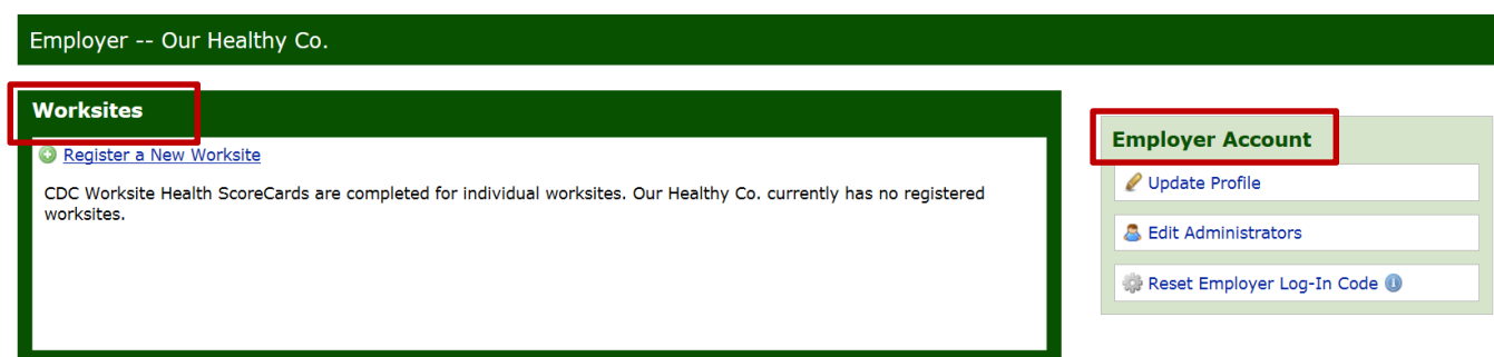
Figure 10: Employer Dashboard
